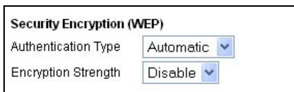
Figure 3-3: Encryption Strength
