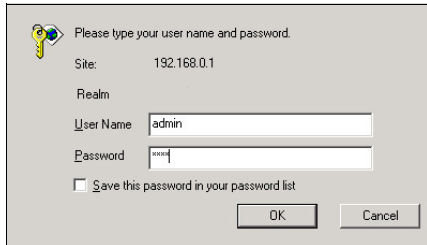
Figure 2-5: Login window
